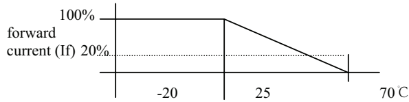
Forward Current Derating Curve
